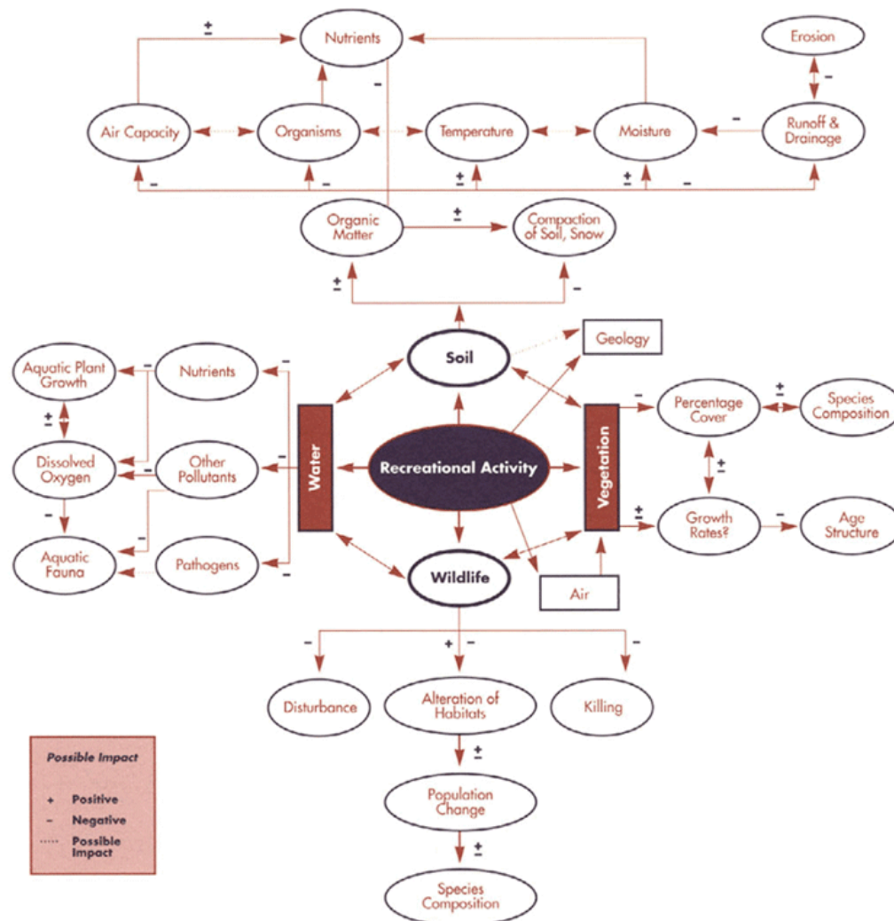
Figure 2. A framework for understanding the ecological effects of recreational activity (Adapted from Mathieson and Wall (1982), in ICLEI and IDRC 1996)
