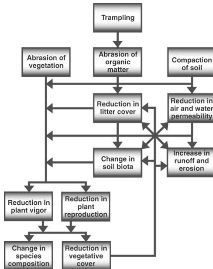
Figure 6. A conceptual model of trampling effects (Therrell et al. 2007)
